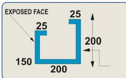
ROOF GUTTER
