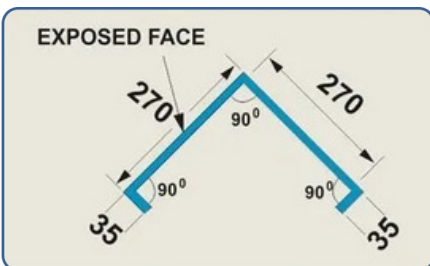
CORNER FLASHING
