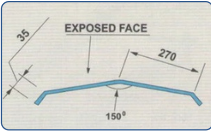
PLAIN RIDGE
