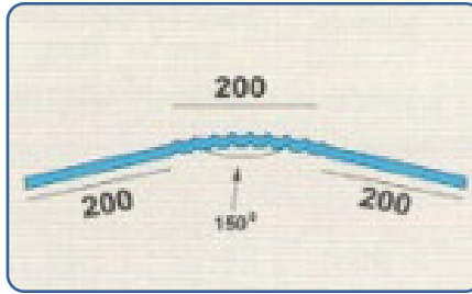
CRIMPED RIDGE
